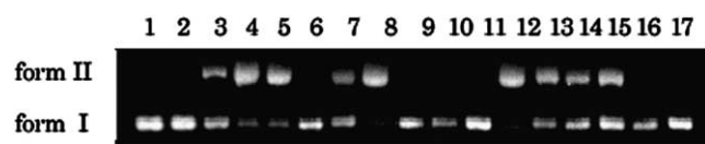
Figure 1. Single-strand cleavage of supercoiled circular \phi X174 RFI DNA (form I, 50 \mu M/base pair, molecular weight 3.50 \times 10^6 , 5386 base pairs in length) to relaxed circular DNA (form II) was carried out by irradiation of a hydrazone (250 \mu M) with 350 nm UV light in a sodium phosphate buffer (pH 6.0) under aerobic conditions at room temperature for 2.0 h. The resultant products were subjected to electrophoresis on 1% agarose gel followed by ethidium bromide staining: lane 1, DNA alone; lane 2, 1 in the dark; lane 3, 1 ; lane 4, 2 ; lane 5, 3 ; lane 6, 4 ; lane 7, 5 ; lane 8, 6 ; lane 9, 7 ; lane 10, 8 ; lane 11, 9 ; lane 12, 10 ; lane 13, 11 ; lane 14, 12 ; lane 15, 13 ; lane 16, 14 ; lane 17, 15 .
